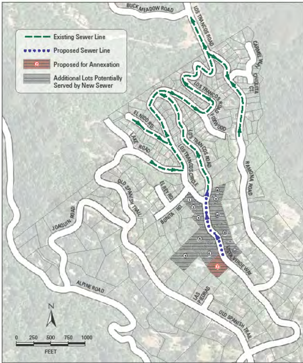
Figure 2 Proposed New Sewer Line and Potential New Service Area
