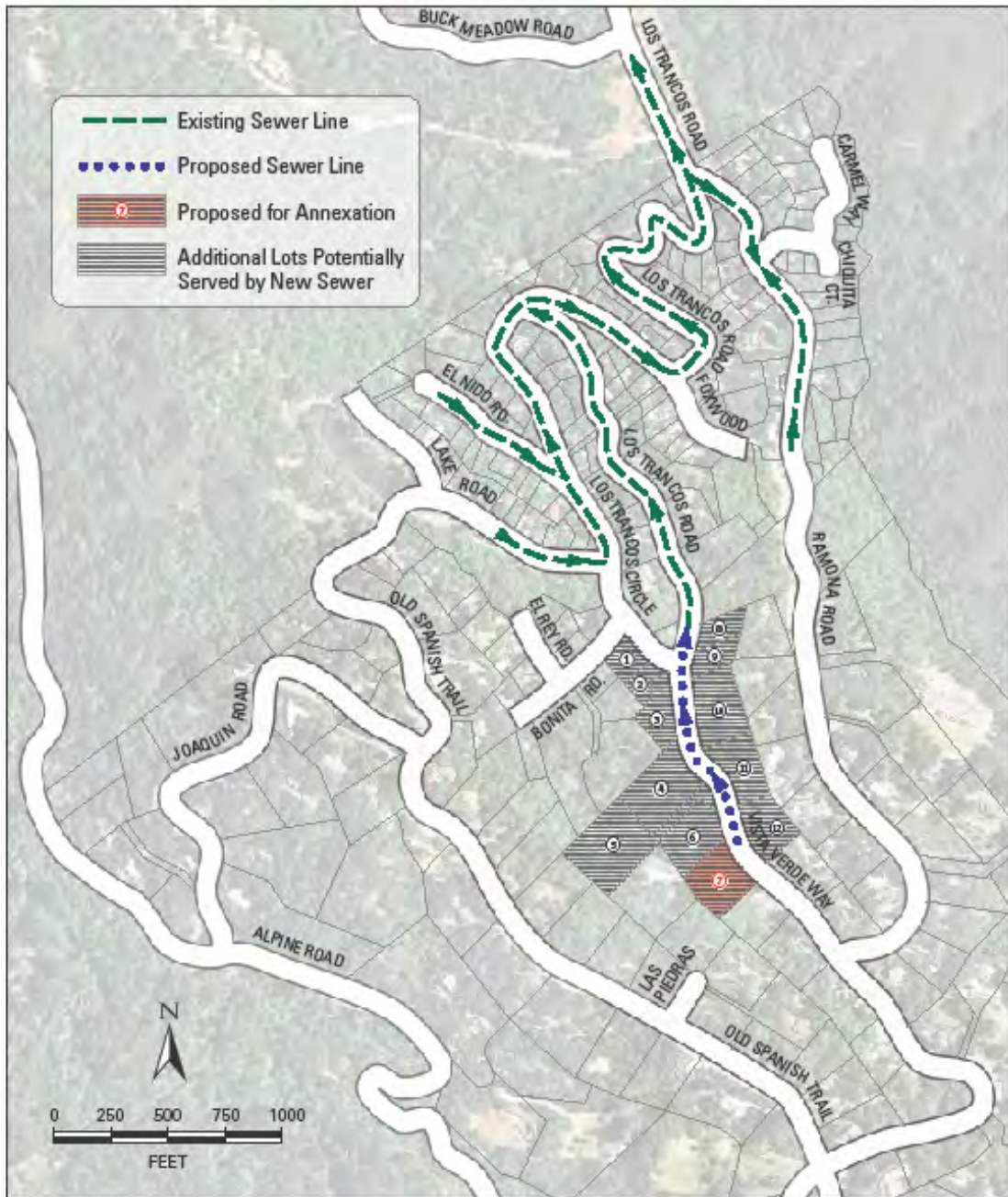
Figure 2 Proposed New Sewer Line and Potential New Service Area
